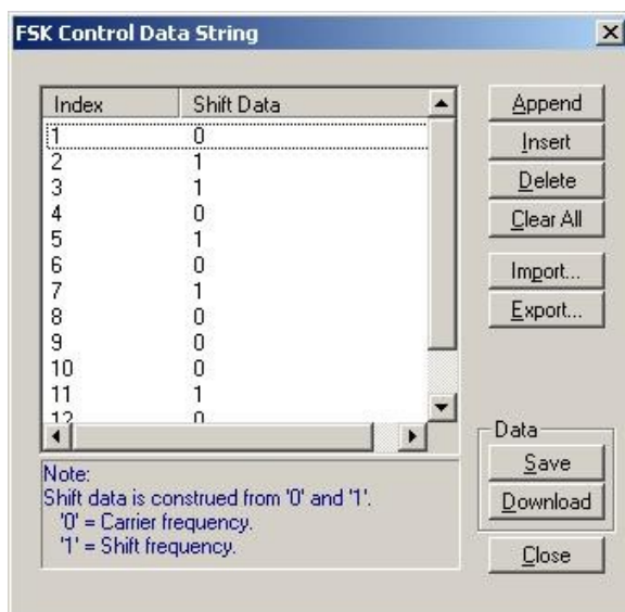
Figure 3-70, FSK Control Data String Example
