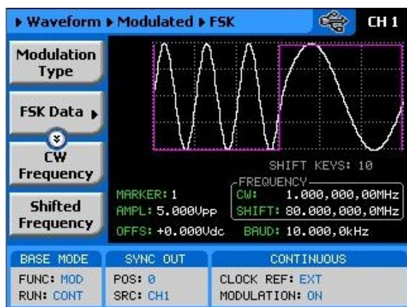
Figure 3-69, FSK Menus
