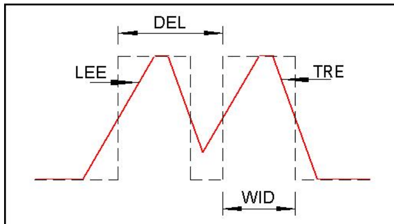
Figure 3-43, Output Waveform with Error 107 (207) Example
