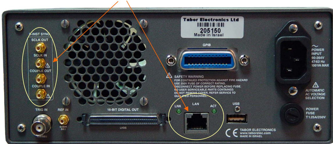
Figure 3-91, Connecting the PM8572 Synchronization Cables
