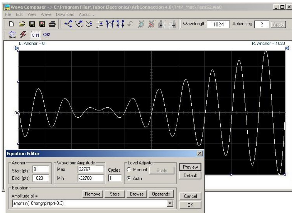
Figure 4-39, the Waveform Screen
