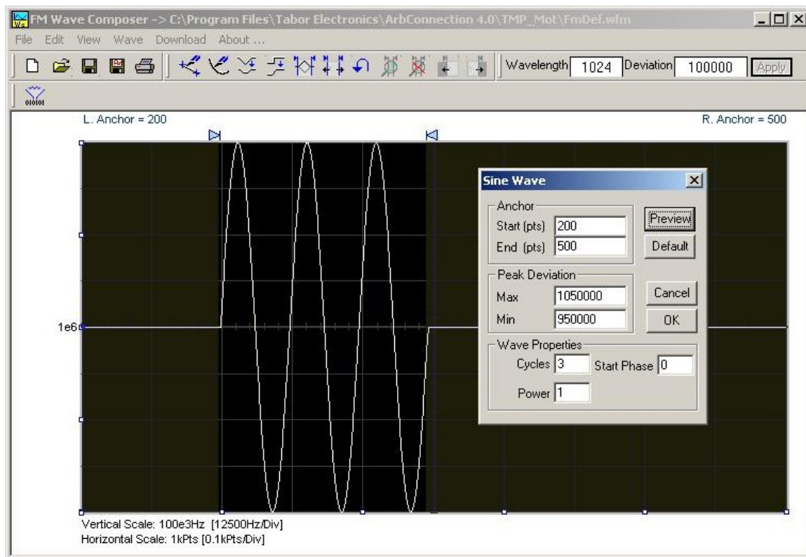
Figure 4-62, Generating Sine Modulation Using the FM Composer
