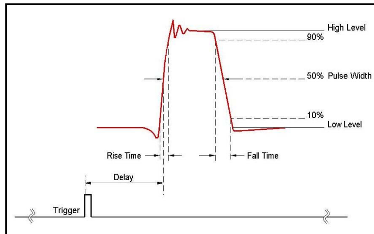
3-22, Delayed Pulse Mode
