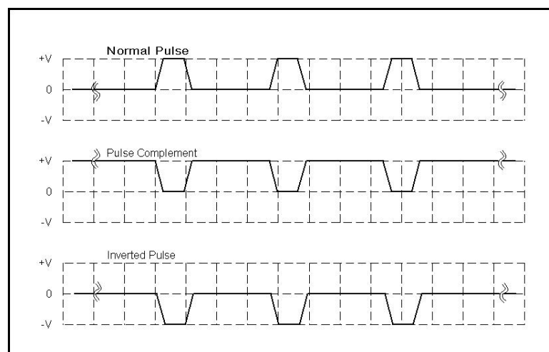
Figure 3-32, Pulse Polarity Options
