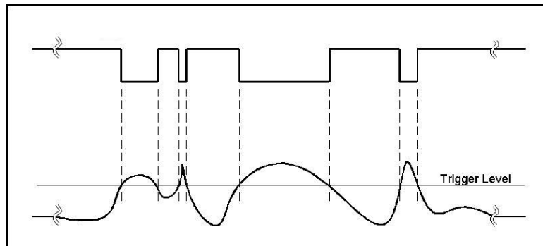
Figure 3-27, External Pulse Width Mode, Negative Slope Example
