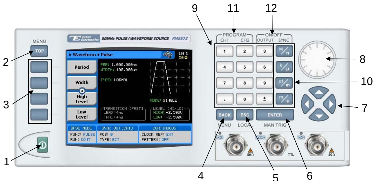
Figure 1-6, PM8572 Front Panel Controls
