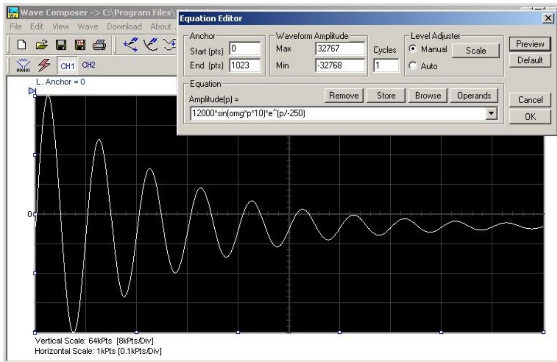
Figure 4-44, Using the Equation Editor to Generate Exponentially Decaying Sinewave
