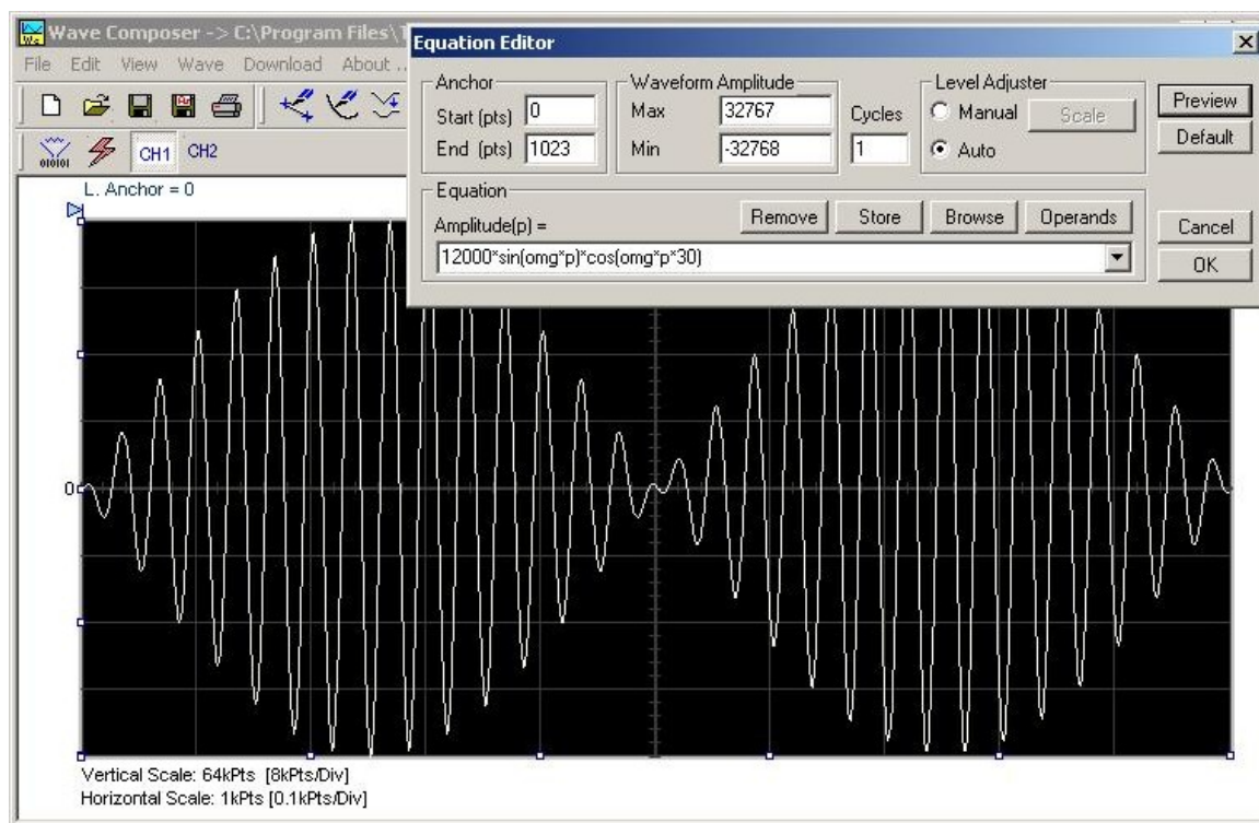
Figure 4-42, Using the Equation Editor to Modulate Sine Waveforms.
