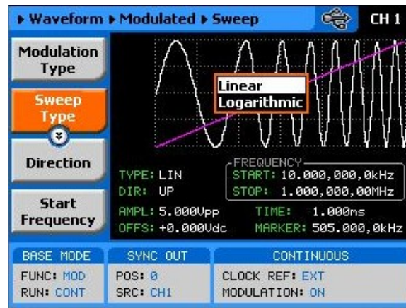
Figure 3-60, Sweep Menus
