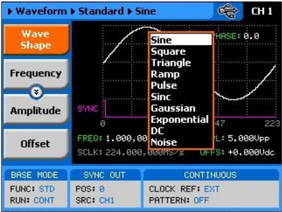
Figure 3-45, Built-in Standard Waveforms Menu
