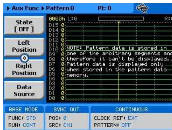
Figure 3-88, Digital Pattern Display while Using the Arbitrary Memory
