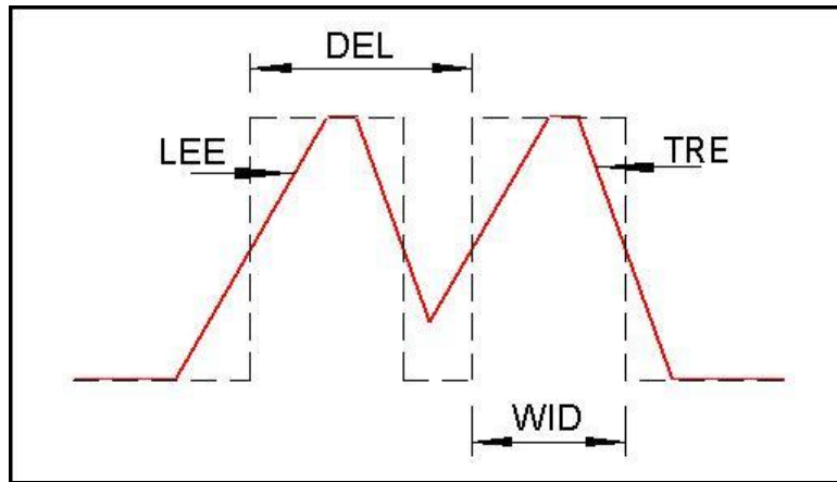
Figure 3-40, Output Waveform with Error 102 (202) Example
