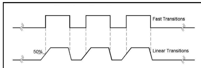
Figure 3-34, Fast and Linear Transitions, Compared
