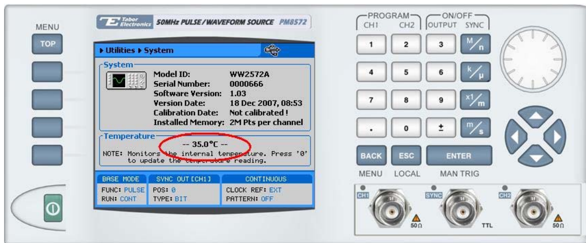
Figure 3-99, Reading the PM8572 Internal Temperature
