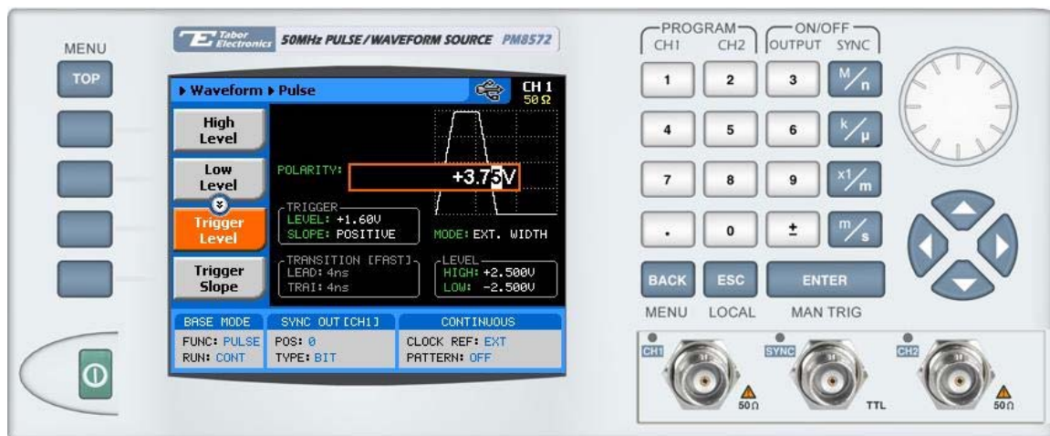
Figure 3-29, External Pulse Width Parameters
