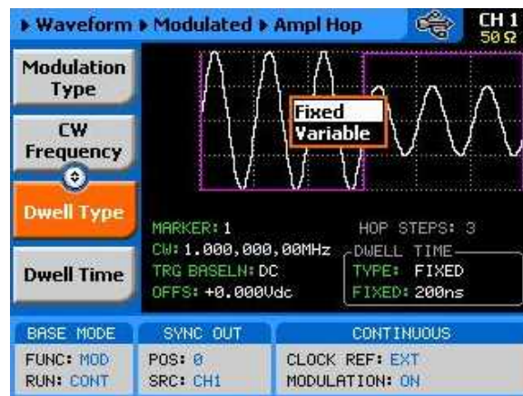
Figure 3-63, Amplitude Hop Menus
