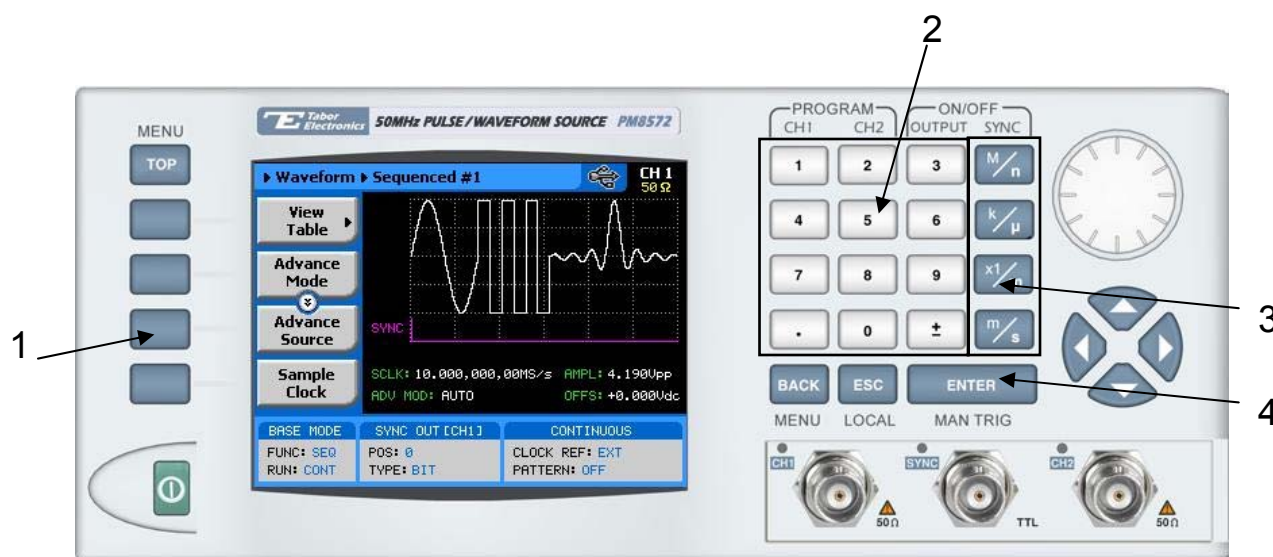
Figure 3-49, Sequence Parameters
