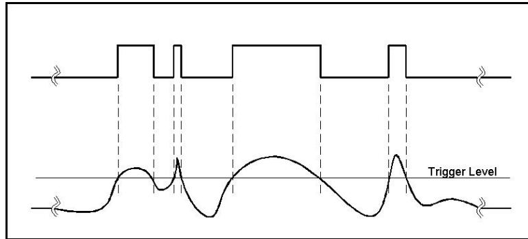
Figure 3-26, External Pulse Width Mode, Positive Slope Example
