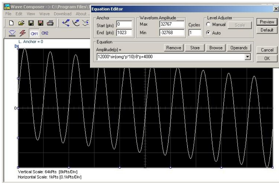
Figure 4-41, an Equation Editor Example
