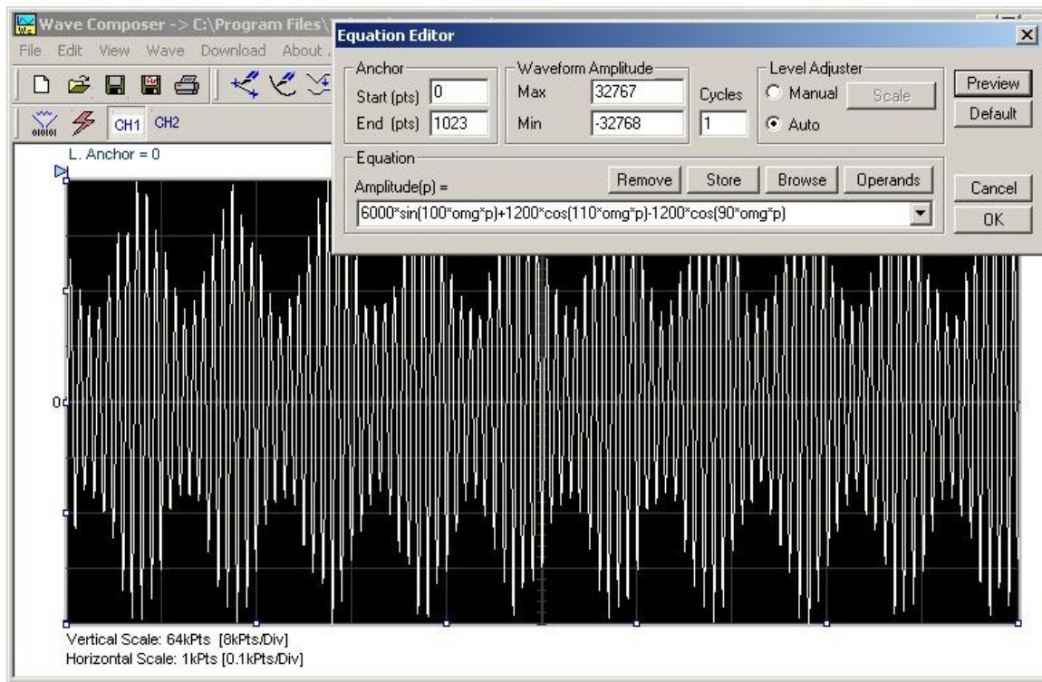
Figure 4-45, Using the Editor to Build Amplitude Modulated Signal with Upper and Lower Sidebands
