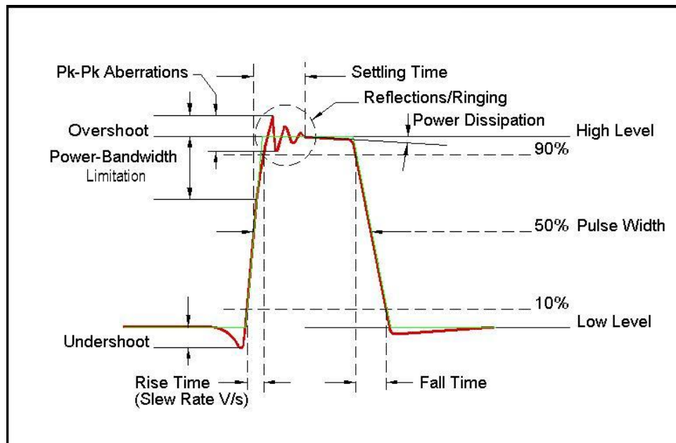
Figure 3-19, Single Pulse Parameters Summary
