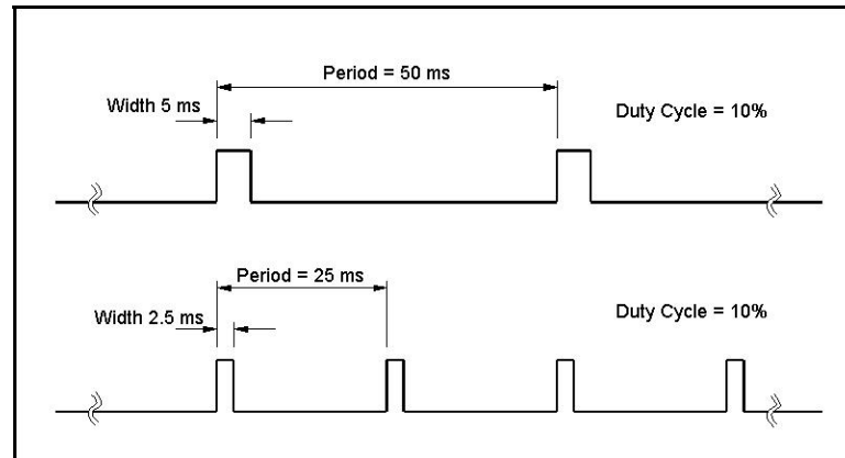
Figure 3-24, Hold Duty Cycle Mode Example
