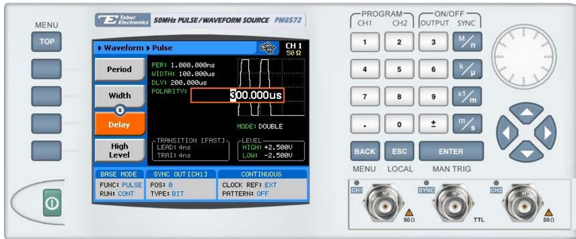
Figure 3-21, Programming the Double Pulse Delay
