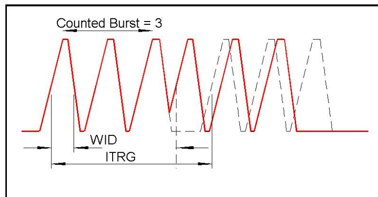
Figure 3-44, Output Waveform with Error 108 (208) Example
