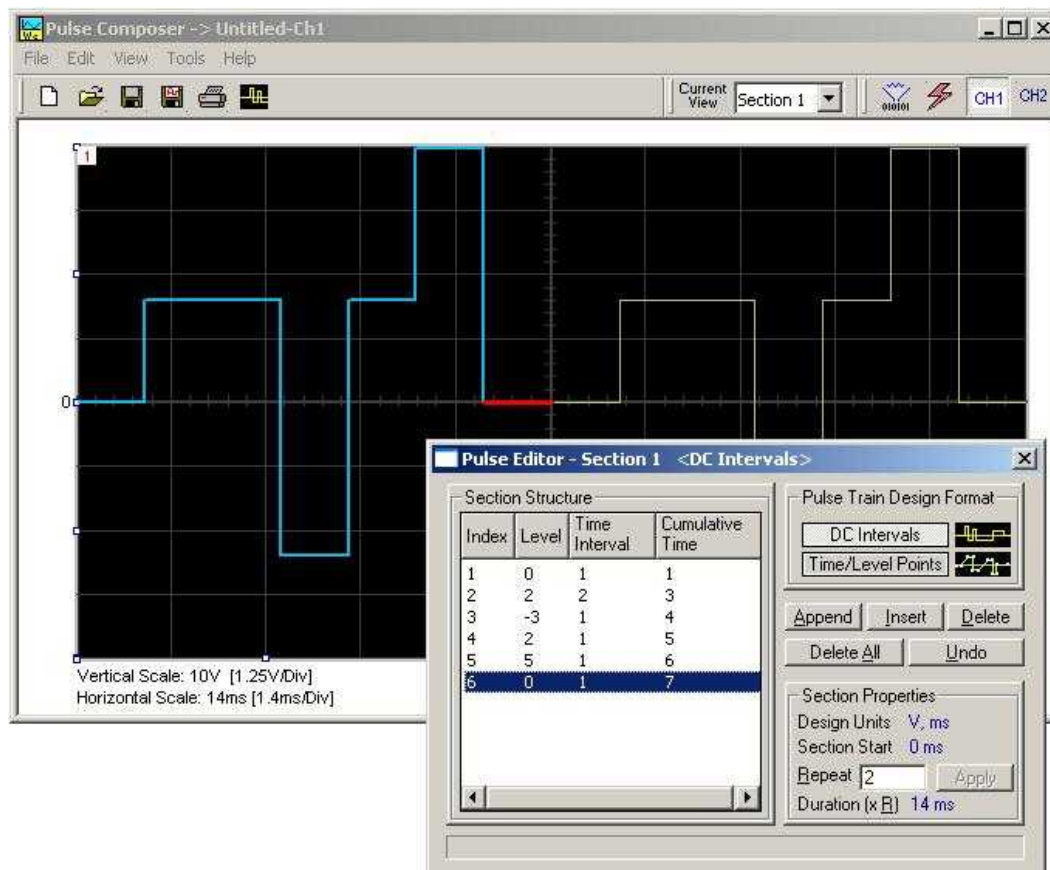
Figure 4-55, Building Section 1 of the Pulse Example
