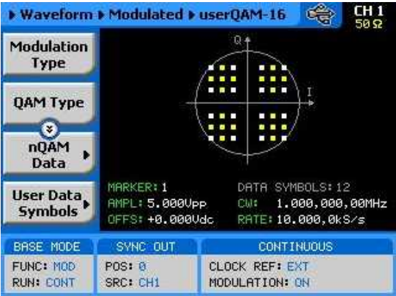
Figure 3-79, User Display
