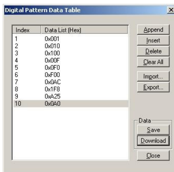
Figure 3-900, Digital Pattern Data Table Example
