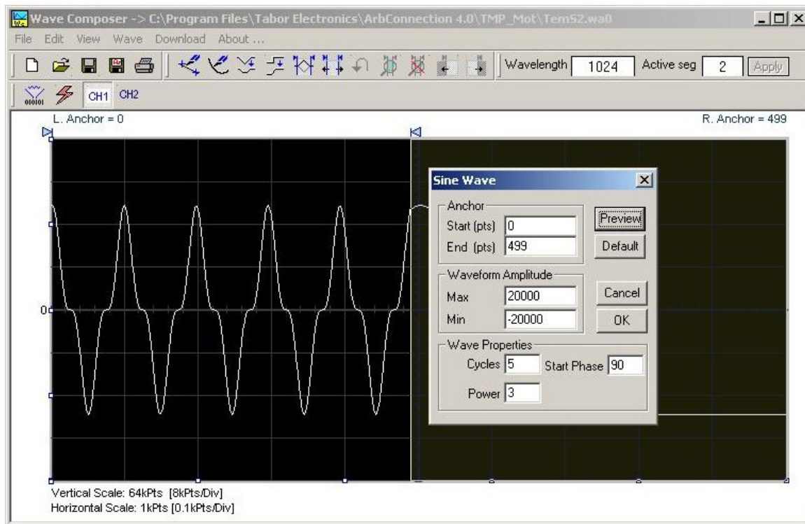
Figure 4-37, Generating Distorted Sine waves from the built-in Library
