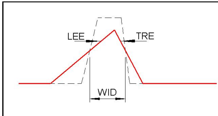
Figure 3-42, Output Waveform with Error 106 (206) Example
