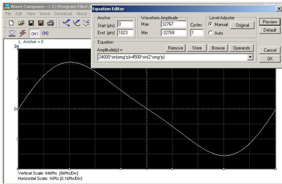
Figure 4-43, Using the Equation Editor to Add Second Harmonic Distortion.
