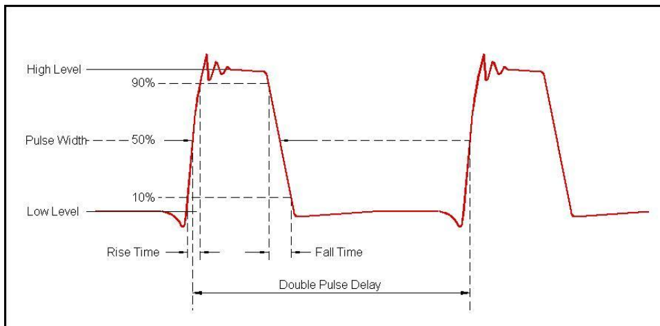
Figure 3-20, Double Pulse Mode
