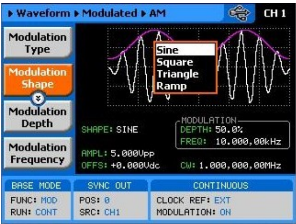
Figure 3-55, Modulating Waveform Shapes
