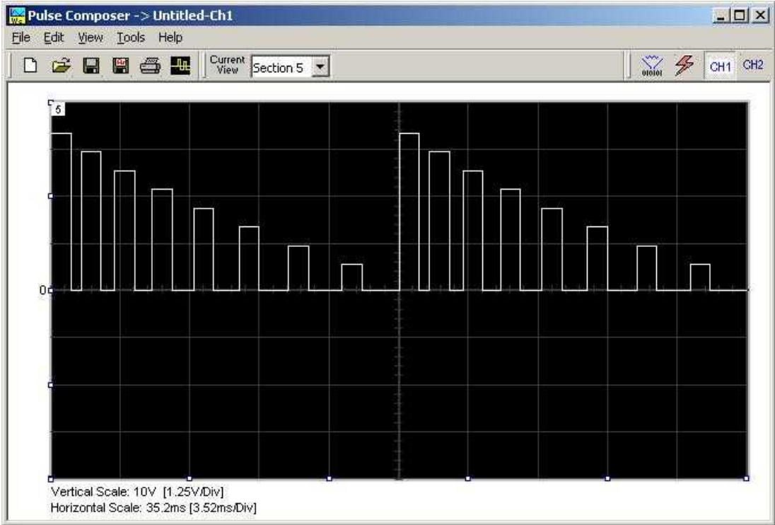
Figure 4-52, Section 5 of the Pulse Train Design
