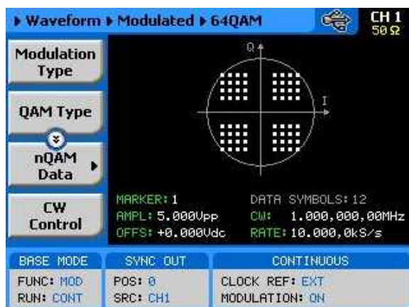
Figure 3-77, 64QAM Display Example
