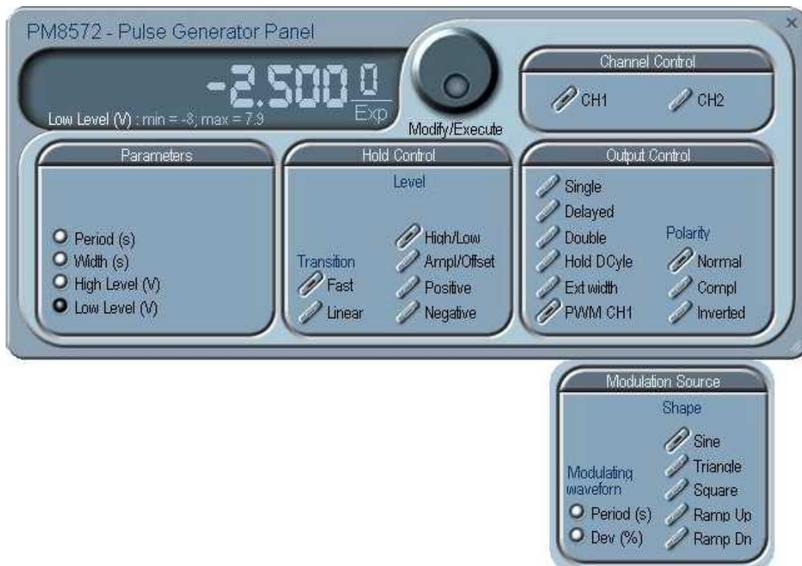
Figure 4-8, PWM Control Parameters
