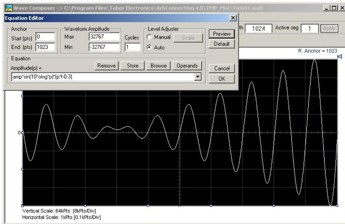
Figure 3-46, the Wave Composer Tool for Generating Arbitrary Waveforms
