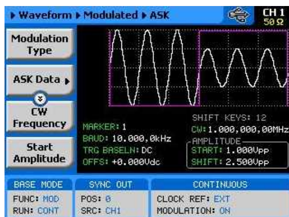
Figure 3-67, ASK Menus
