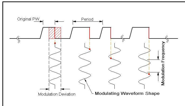
Figure 3-30, Pulse Width Modulation Example
