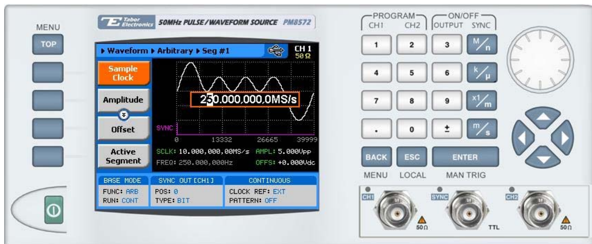
Figure 1-12, Typical PM8572 Arbitrary Waveforms Display
