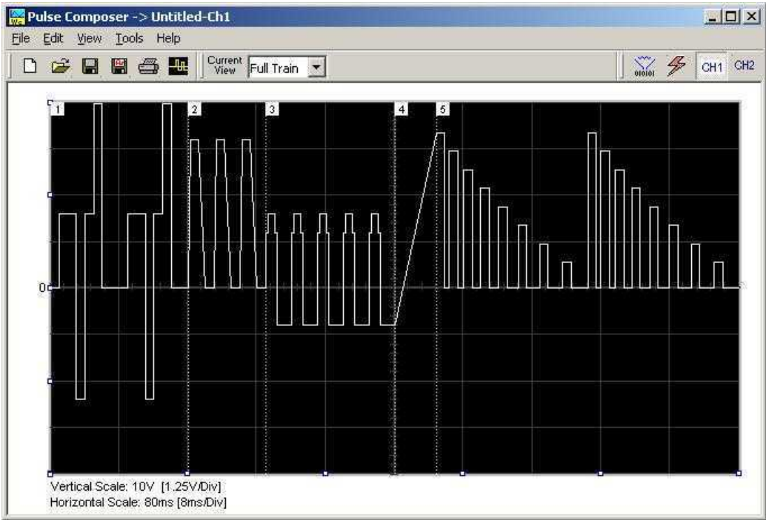
Figure 4-51, Complete Pulse Train Design
