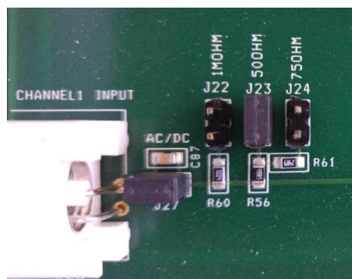
Figure 2-1, Field Modification of Channel 1 Input Impedance
