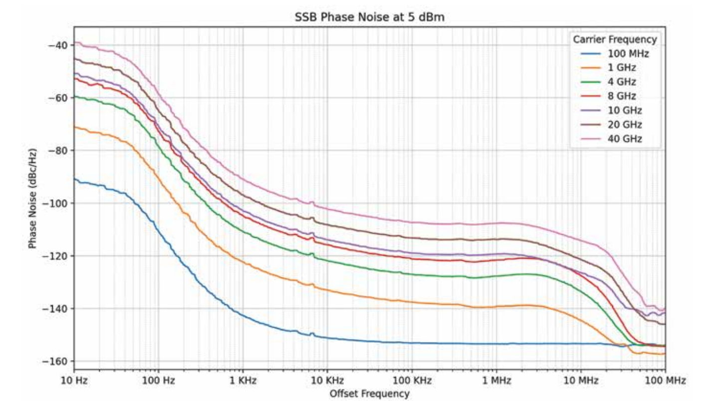
Figure 2: Phase Noise vs. Frequencies at 5 dBm
