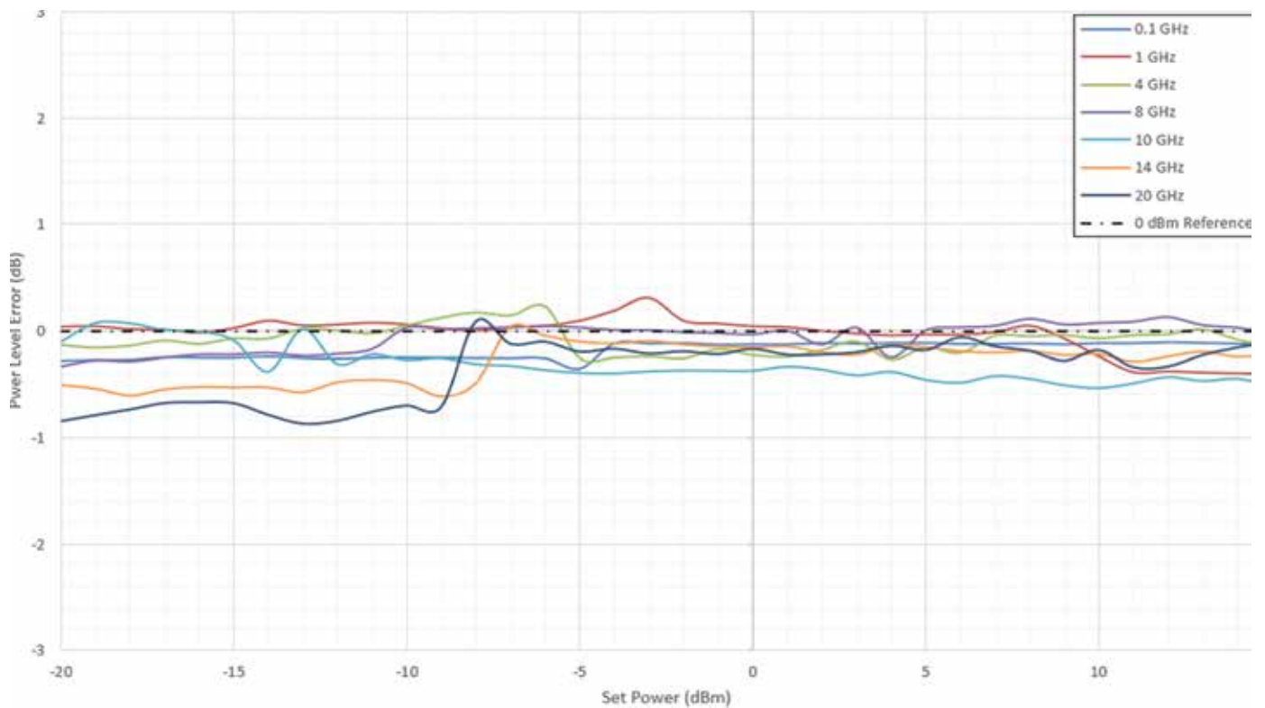
Figure 8: Power Linearity over Frequencies up to 20 GHz
