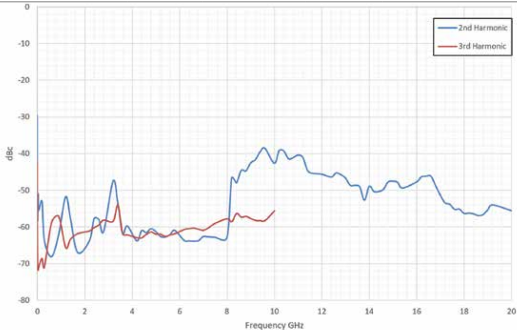
Figure 3: Harmonics at 0 dBm
