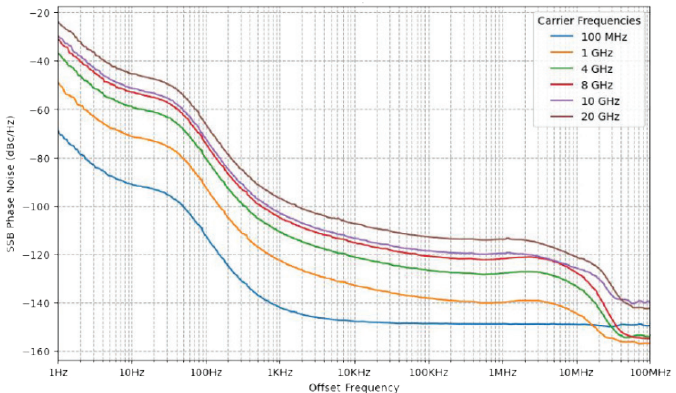
Figure 2: Phase Noise vs. Frequencies at 0 dBm
