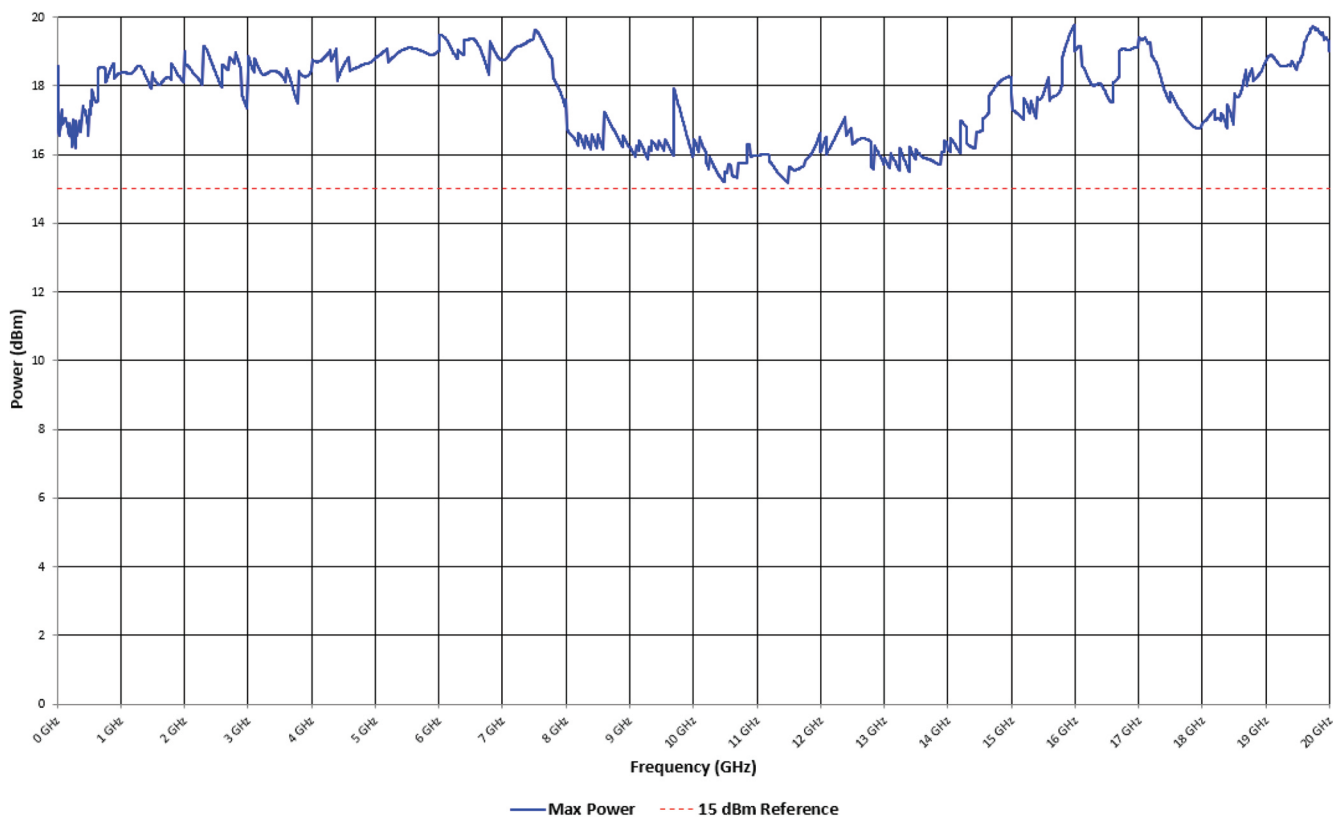
Figure 6: Max Power vs. Frequency up to 20 GHz
