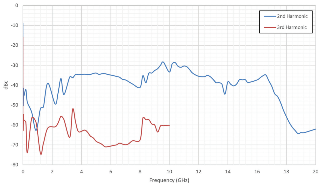
Figure 5: Harmonics at 10 dBm
