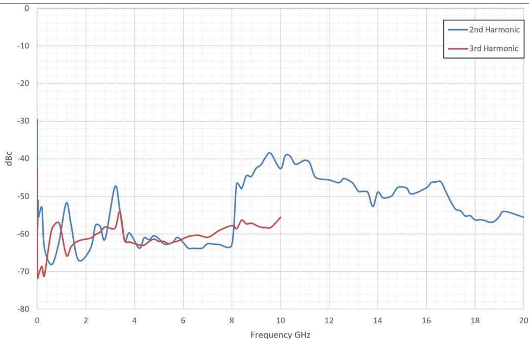
Figure 4: Harmonics at 5 dBm
