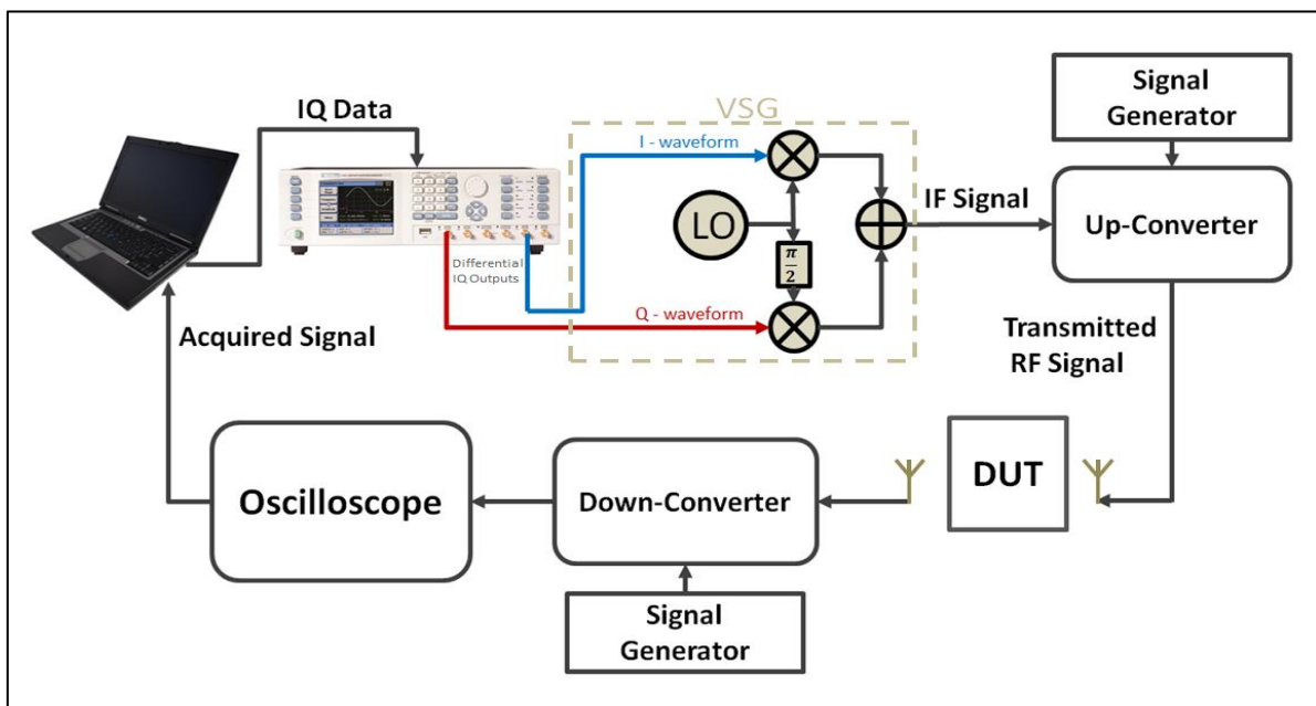
Figure 5: Creation of I/Q signals for a VSG using Tabor SE5082 AWG
