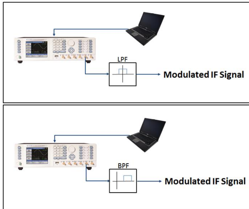
Figure 6: (a) Direct RF/IF generation using LPF for first Nyquist band. (b) Direct RF/IF generation using BPF for a higher Nyquist band
