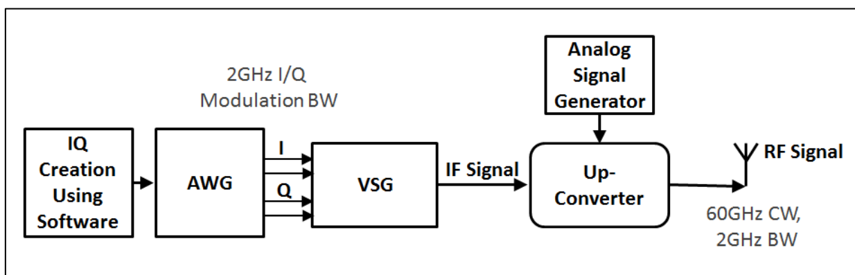
Figure 4: Typical WiGig receivers test setup using an AWG
