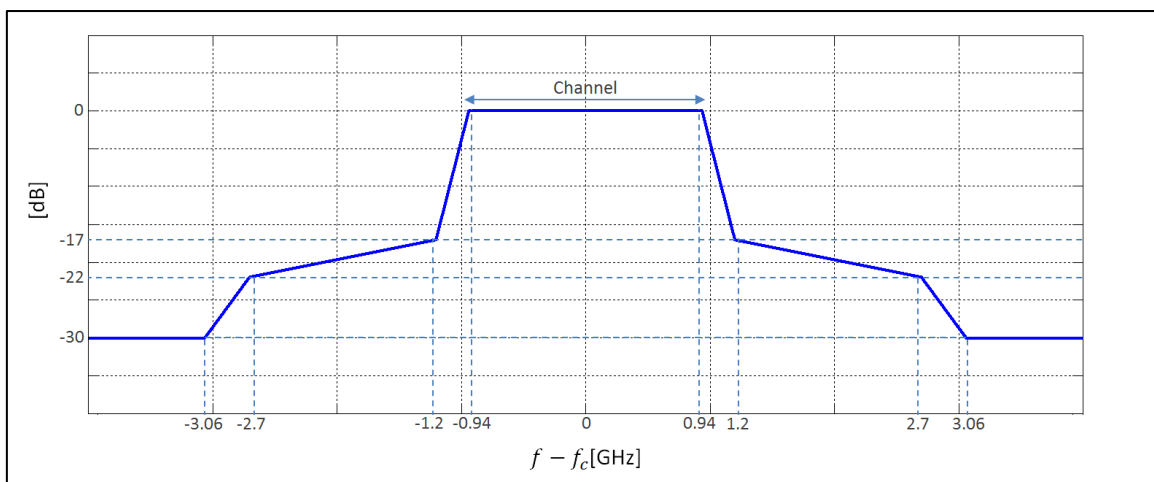
Figure 2: Spectral Mask of 802.11ad packet with RBW of 1MHz.
