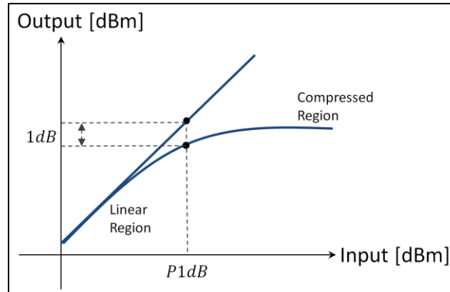
Figure 3: 1dB compression point
